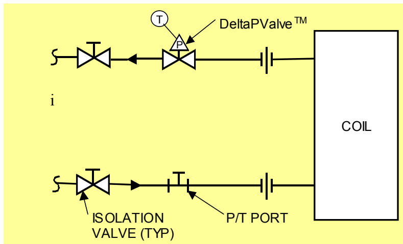
Figure 8: DeltaPValve with Typical Coil
