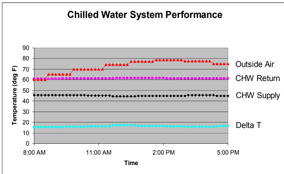
Figure 2: Building Chilled Water Performance Trend
