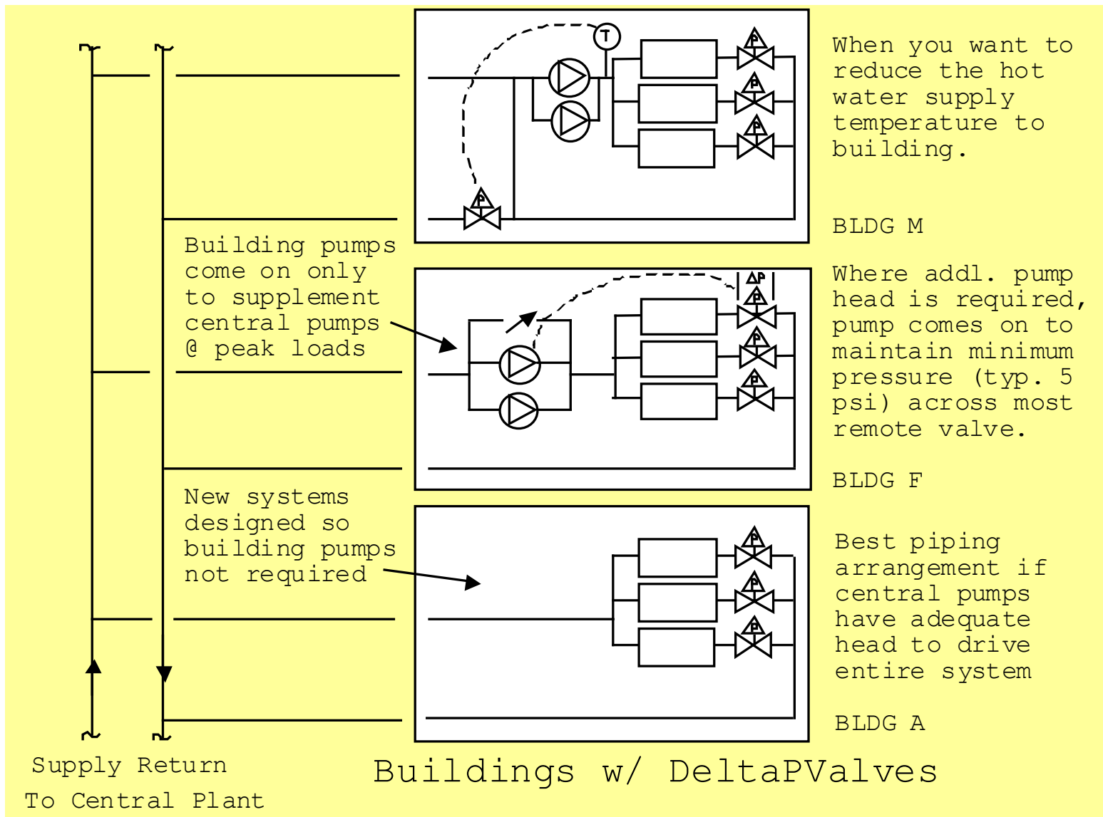
Figure A3: Buildings on Large Heating or Cooling Distribution System
