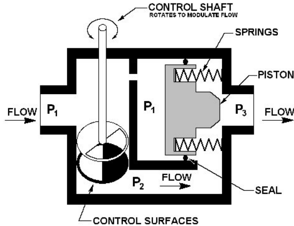
Figure 6: DeltaP Valve Schematic
