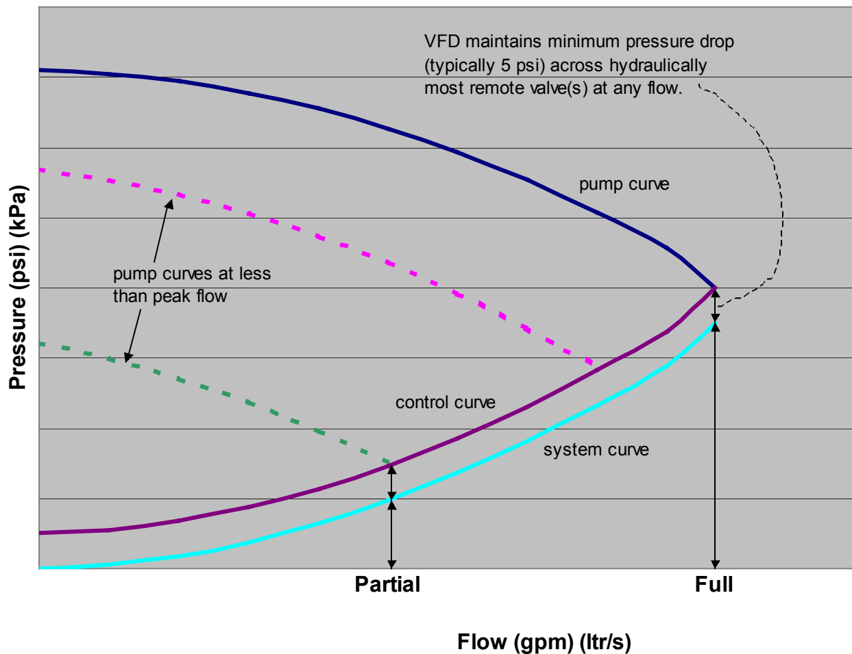
Figure 5: Variable Speed Pumping
