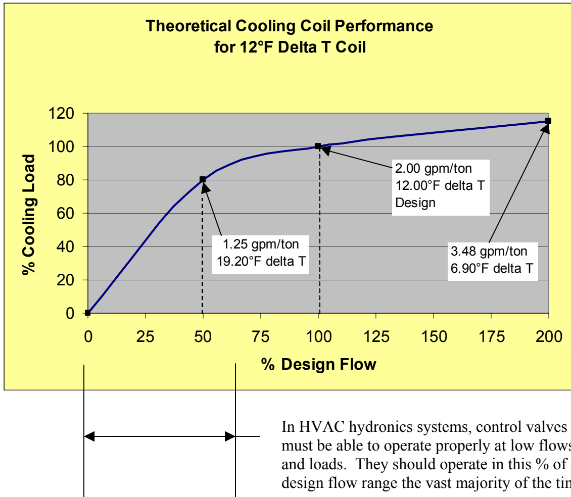
Figure 3: Cooling Coil Theoretical Performance
