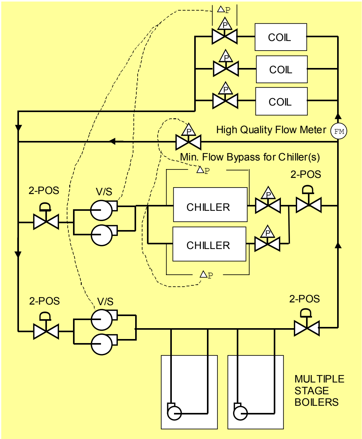
Figure A9: Two-Pipe Changeover System – Excellent System for Schools
