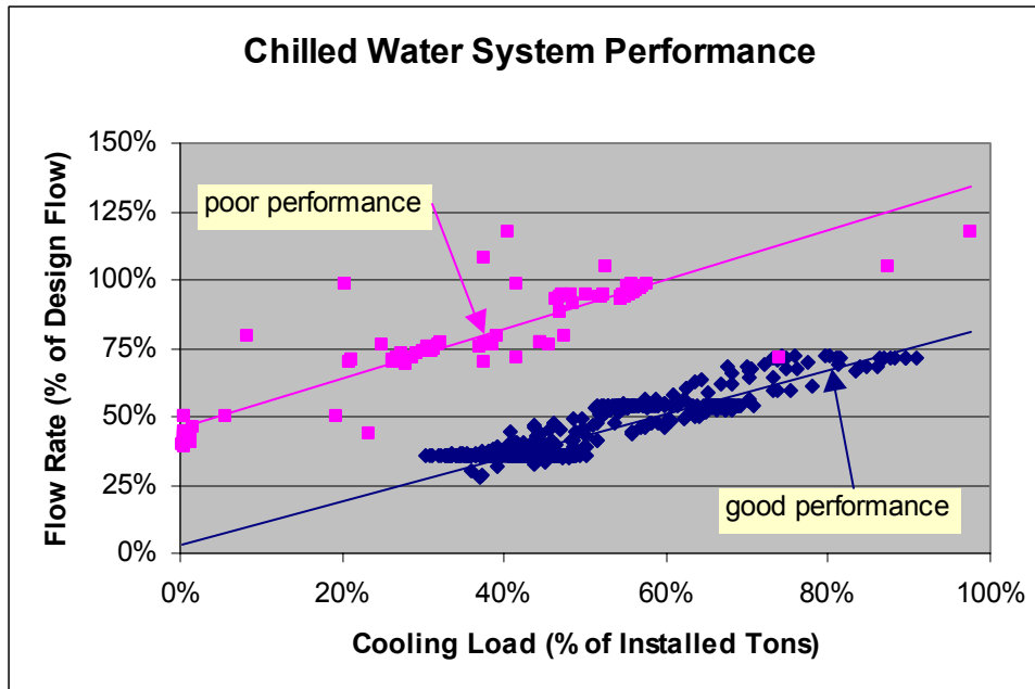
Figure 1: % Cooling Load vs. % Flow Rate
