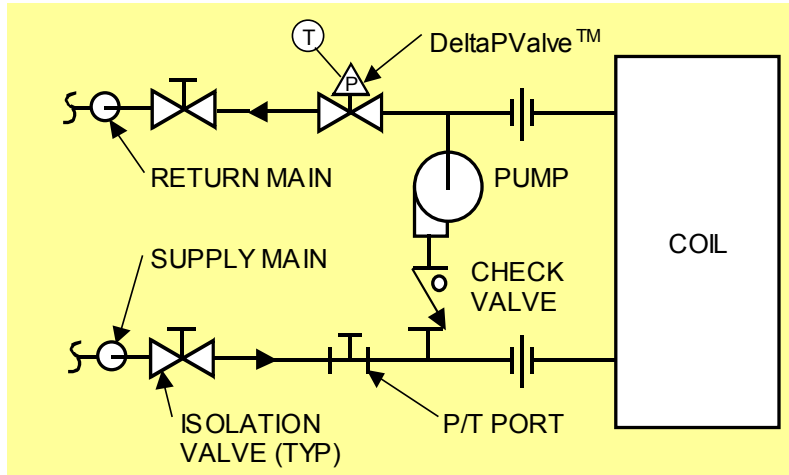
Figure 9: Pumped Coil Schematic
