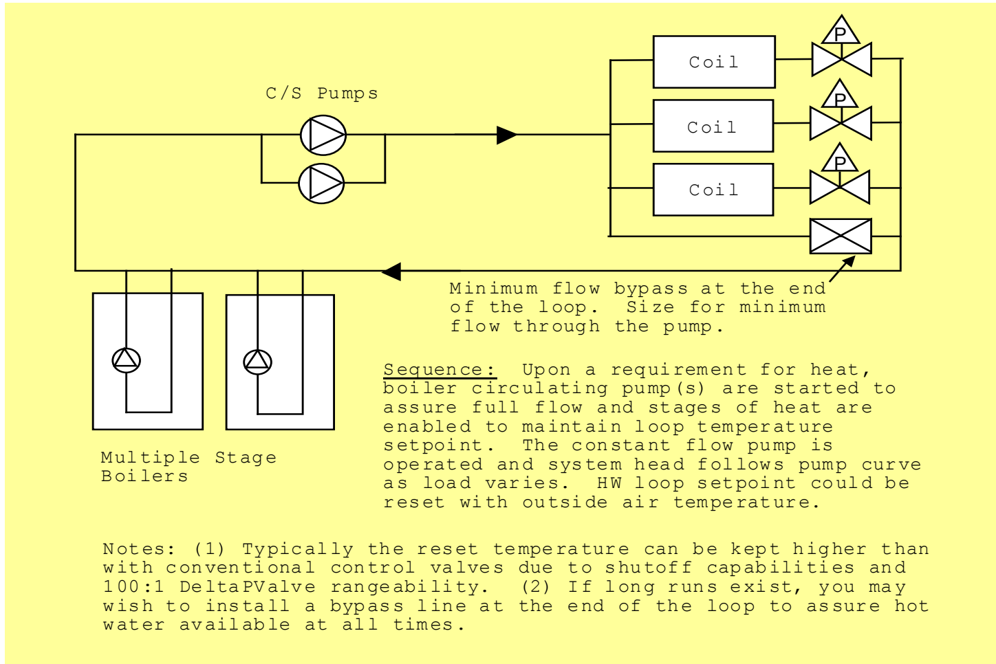
Figure A1: Small Heating System - Constant Speed Pump
