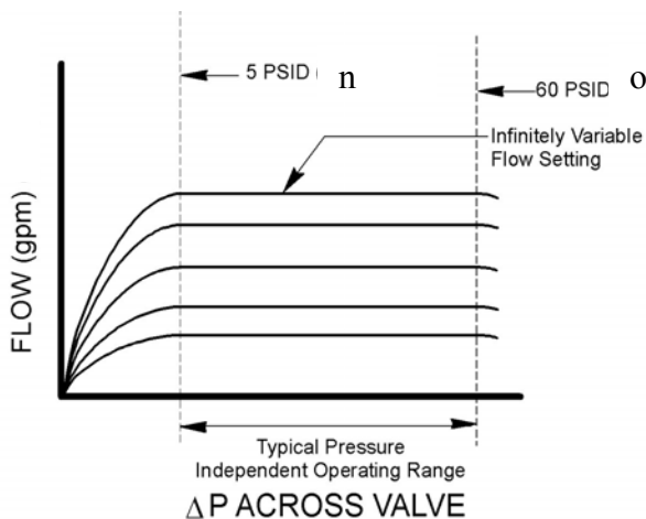
Figure 7: DeltaP Valve Performance
