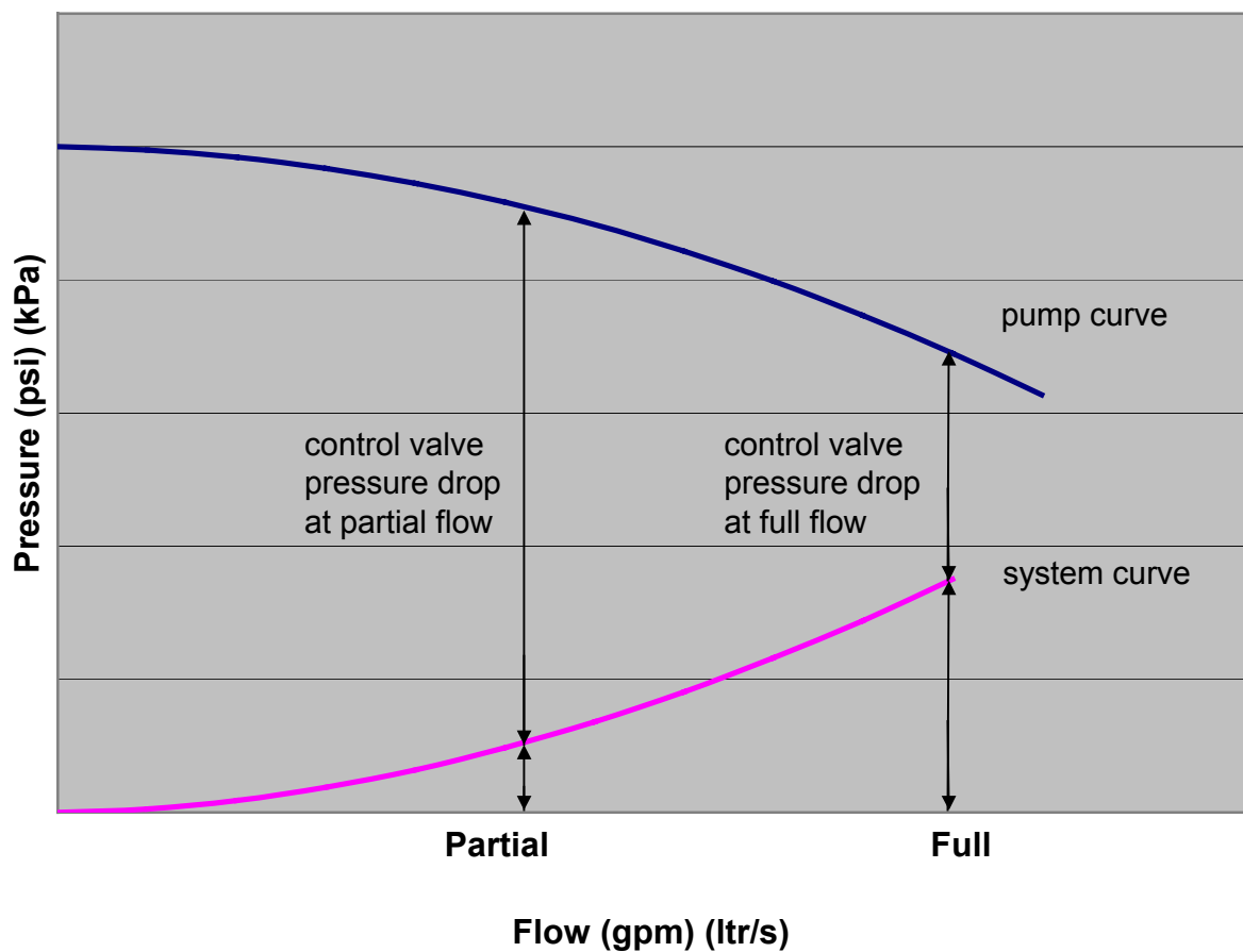
Figure 4: Constant Speed Pumping
