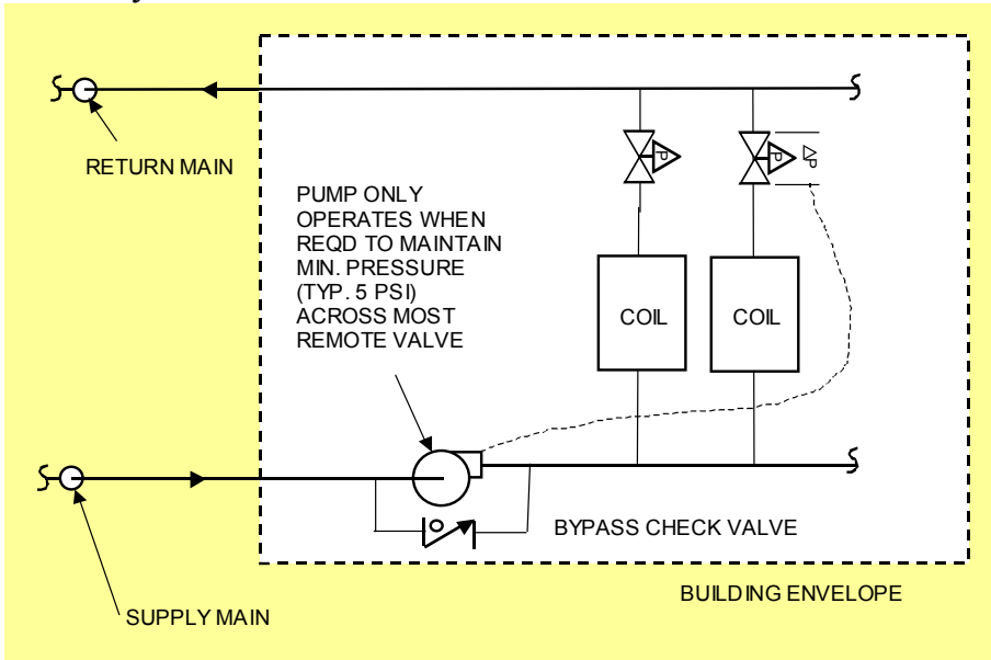
Figure A10: To Address Humidity Issues in Decoupled Laboratory, Hospital, and Other Buildings
